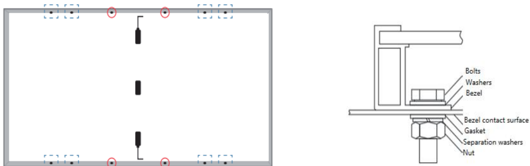
Figure 2 Schematic diagram of single-sided component mounting holes (The remaining component mounting holes are shown in the corresponding component layout)
