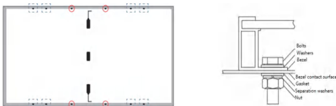
Figure 2 Schematic diagram of single-sided component mounting holes
