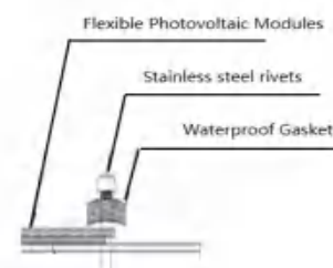
Figure 4: Schematic diagram of flexible component mounting holes
