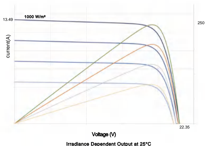
RSP250DCT Characteristics Versus Voltage
