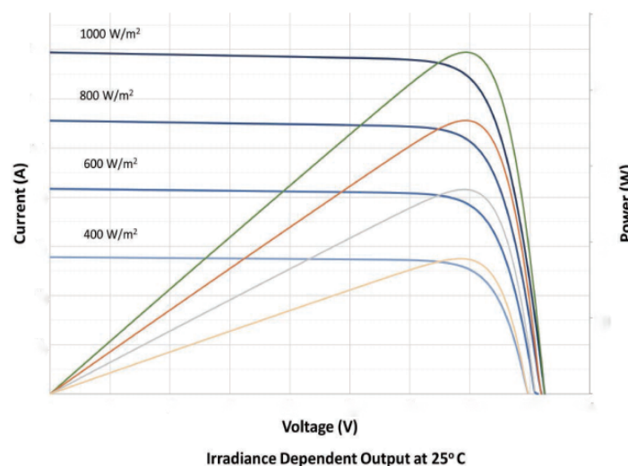
RSP150MCB-BB-T-G1- Characteristics Curve
